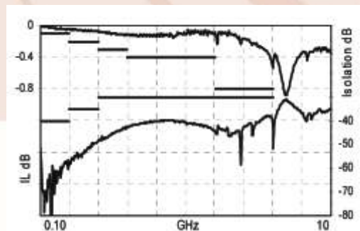
Typical ISOLATION and INSERTION LOSS
