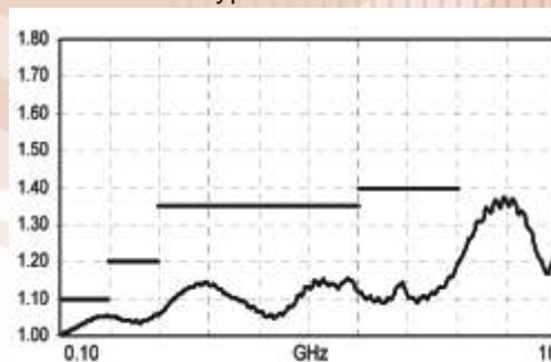
Typical V.S.W.R.
